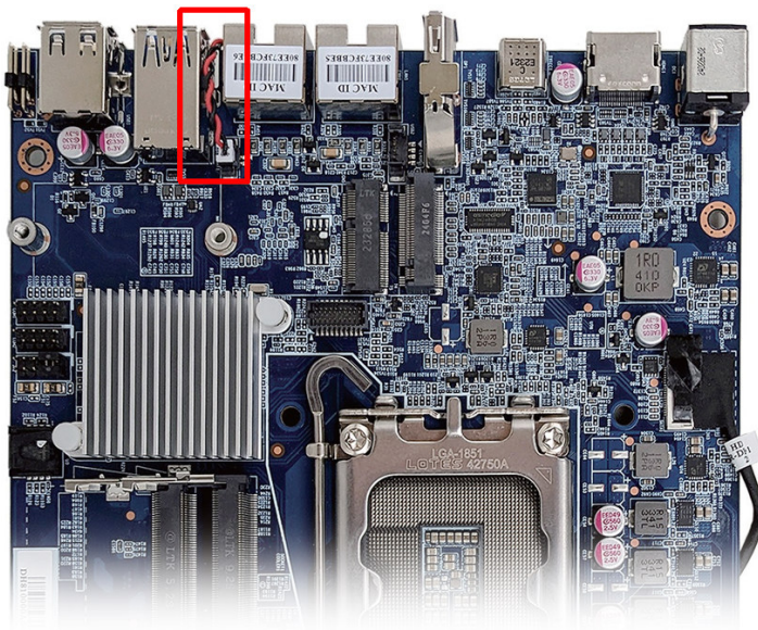
Photo: Position of the button cell battery and the connector on the mainboard.
