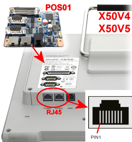
POS01 pin assignment of COM3/COM4 port with RJ45 output connector:
