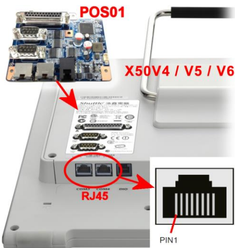
POS01 pin assignment of COM3/COM4 port with RJ45 output connector:
