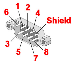
Pin assignment of the 9-pin D-Sub connector
